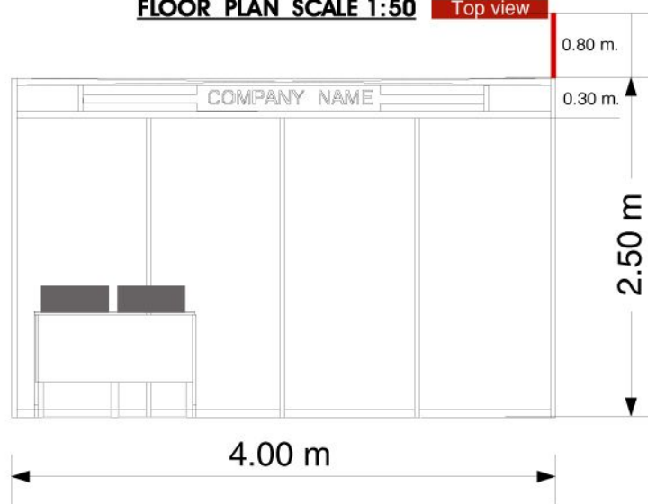
ELEVATION SCALE 1:50 Front view
