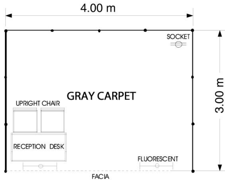
FLOOR PLAN SCALE 1:50 Top view
